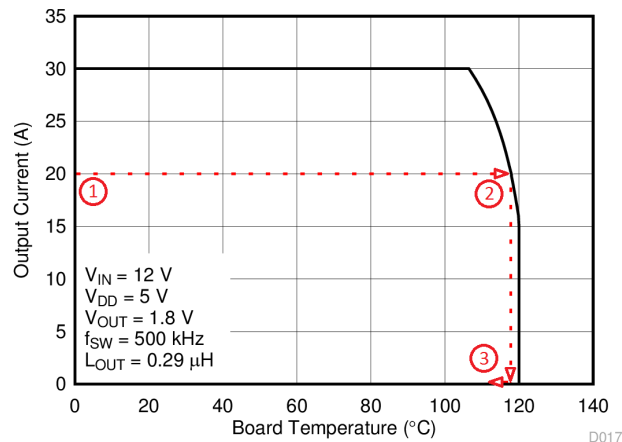
Figure 15. Power Stage CSD97396Q4M SOA
